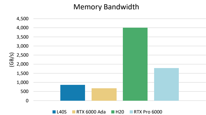
Exhibit 7: While H20 possesses greater memory bandwidth
