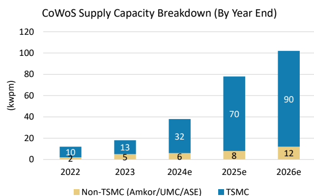
Exhibit 11: Global CoWoS capacity expansion by year end and by vendor
