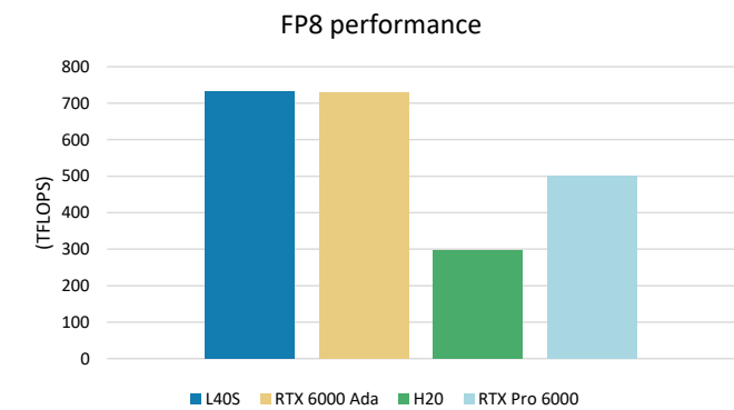
Exhibit 6: L40S and RTX 6000 series products all have better FP8 performance than H20
